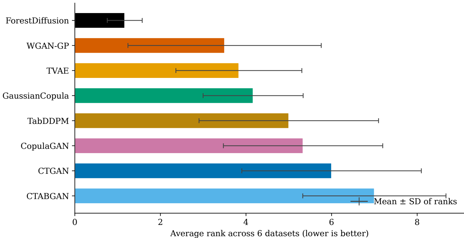
Generator Robustness — Average R 2 -Gap Rank (10-seed means)
